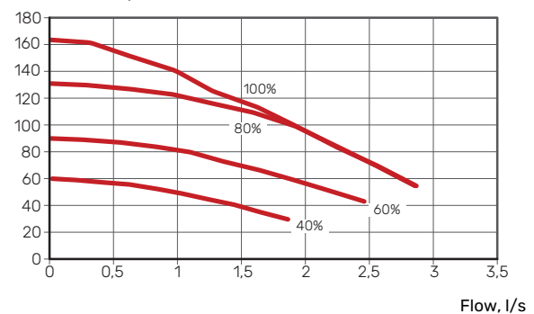
External available pressure (kPa)
