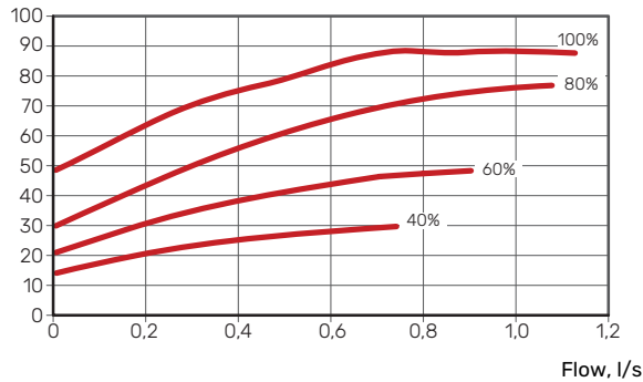
Electrical output per circulation pump (W)
