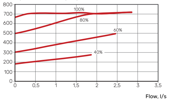
Electrical power, circulation pump (W)
